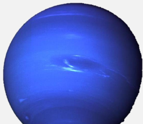
Neptune
