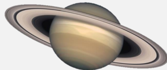
Saturne
